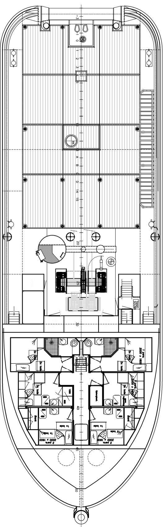
MAIN DECK/TWEEN DECK
