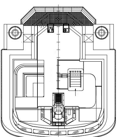
BRIDGE DECK
